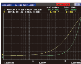
Frequency sweep measurement Z- \theta measurement screen
