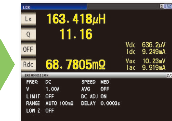
L/Q/ Rdc continuous measurement screen (1 kHz, 1 mA constant current measurement) and Rdc (DC measurement) display screen
